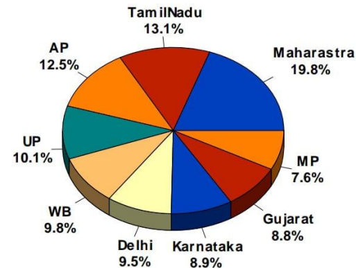
Fig 2 State wise E-waste Generation in India (Tonnes/year)
