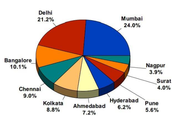
Fig 3 City wise E-waste Generation in India(Tonnes/year)
